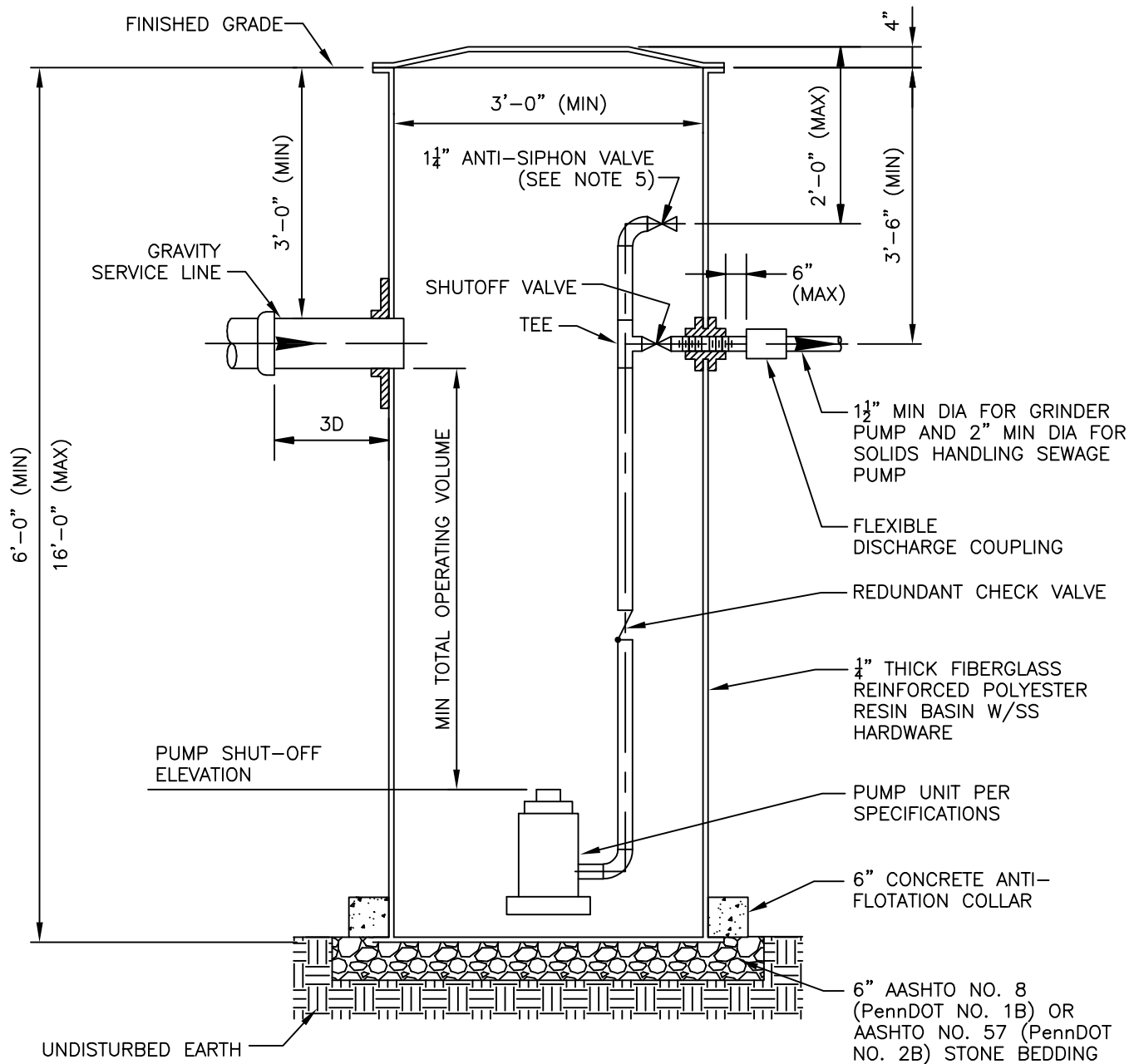
FIBERGLASS BASIN FOR TYPICAL INDIVIDUAL PUMP
