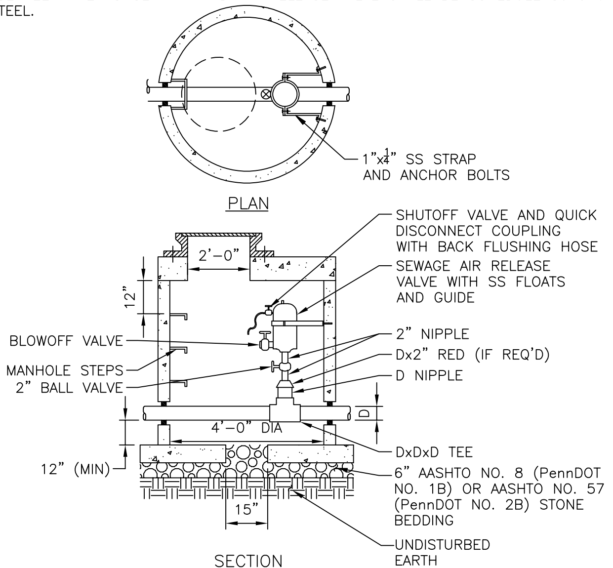
AIR RELEASE VALVE AND CHAMBER
