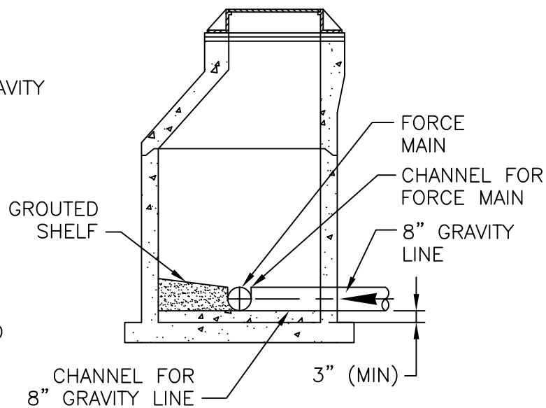
SECTION
