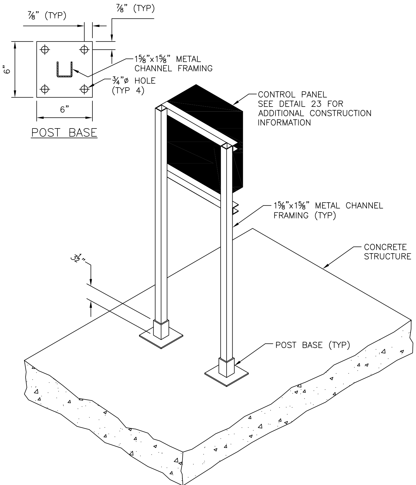
METAL CHANNEL FRAMING FOR CONTROL PANEL MOUNTED ON A CONCRETE STRUCTURE
